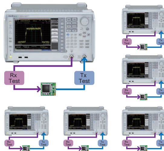
Use "Golden Unit" Signal for Manufacturing Test and Calibration
